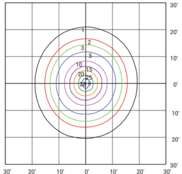
FW4-LED60A40-B-VK-DIM-SP10 (60W 5000K 120V) MOUNTED AT 10 FEET
