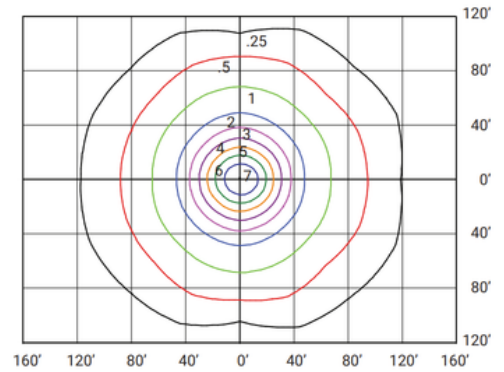
JAG3S-LED430A300-B-VK-VD1-BRZ-DIM-PC-SP10 (430W, 5000K, TYPE V) MOUNTED AT 40 FEET
