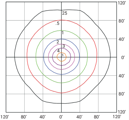
JAG2S-LED300A240-B-VK-VD1-BRZ-DIM-SP10 (300W, 4000K, TYPE V) MOUNTED AT 40 FEET
