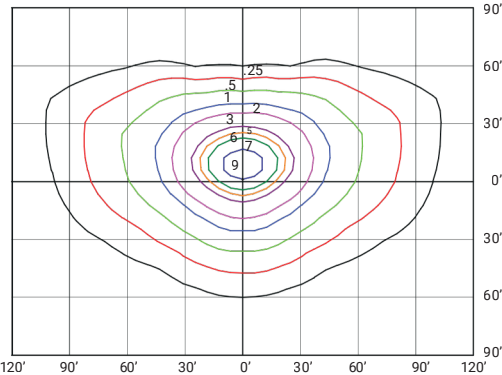
JAG2S-LED240A180-B-VK-VD1-BRZ-DIM-SP10 (240W, 4000K, TYPE III) MOUNTED AT 30 FEET
