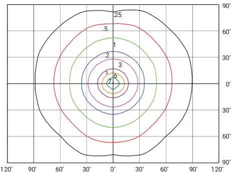
JAG2S-LED300A240-B-VK-VD1-BRZ-DIM-SP10 (300W, 4000K, TYPE V) MOUNTED AT 40 FEET
