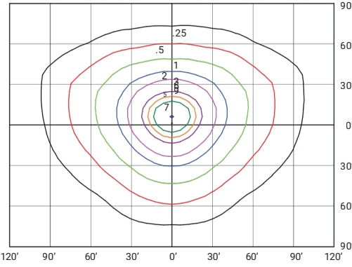
JAG2S-LED300A240-B-VK-VD1-BRZ-DIM-SP10 (300W, 4000K, TYPE IV) MOUNTED AT 40 FEET
