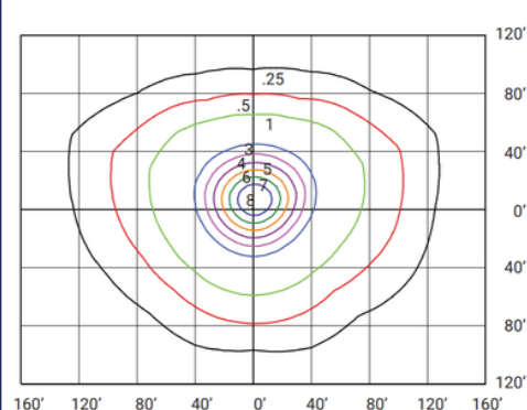
JAG3S-LED430A300-B-VK-VD1-BRZ-DIM-PC-SP10 (430W, 5000K, TYPE IV) MOUNTED AT 40 FEET
