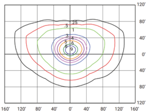
JAG3S-LED430A300-B-VK-VD1-BRZ-DIM-PC-SP10 (430W, 5000K, TYPE III) MOUNTED AT 40 FEET
