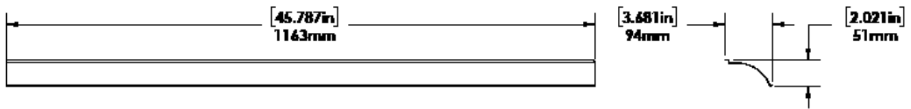
Reflector Wings Kit dimensions
